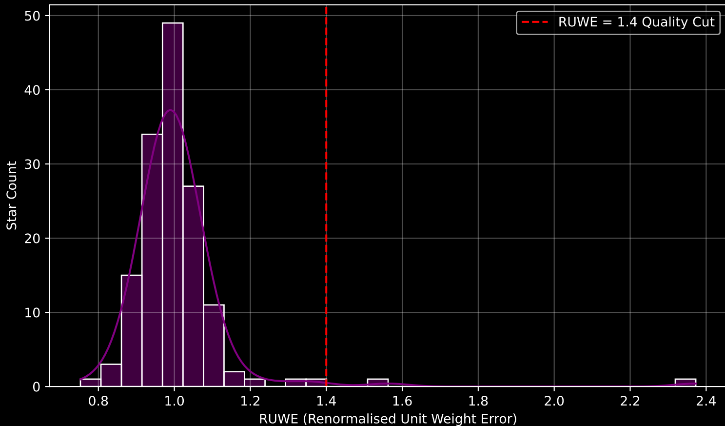
GAPOGEE DR17 Field [356+12-O] RUWE Distribution (n= 147)
