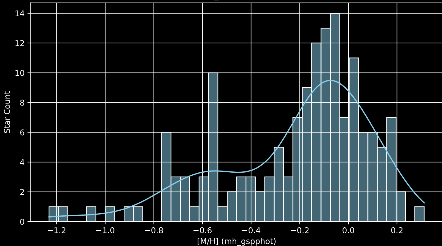
APOGEE DR17 Field: [356+12-O [M/H] (mh_gspphot) (n= 154)
