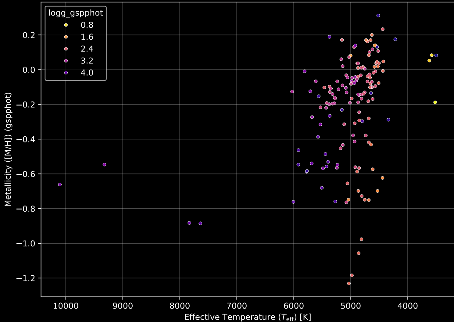
APOGEE DR17 Field: [356+12-O] Stellar Population Parameters (n= 154)
