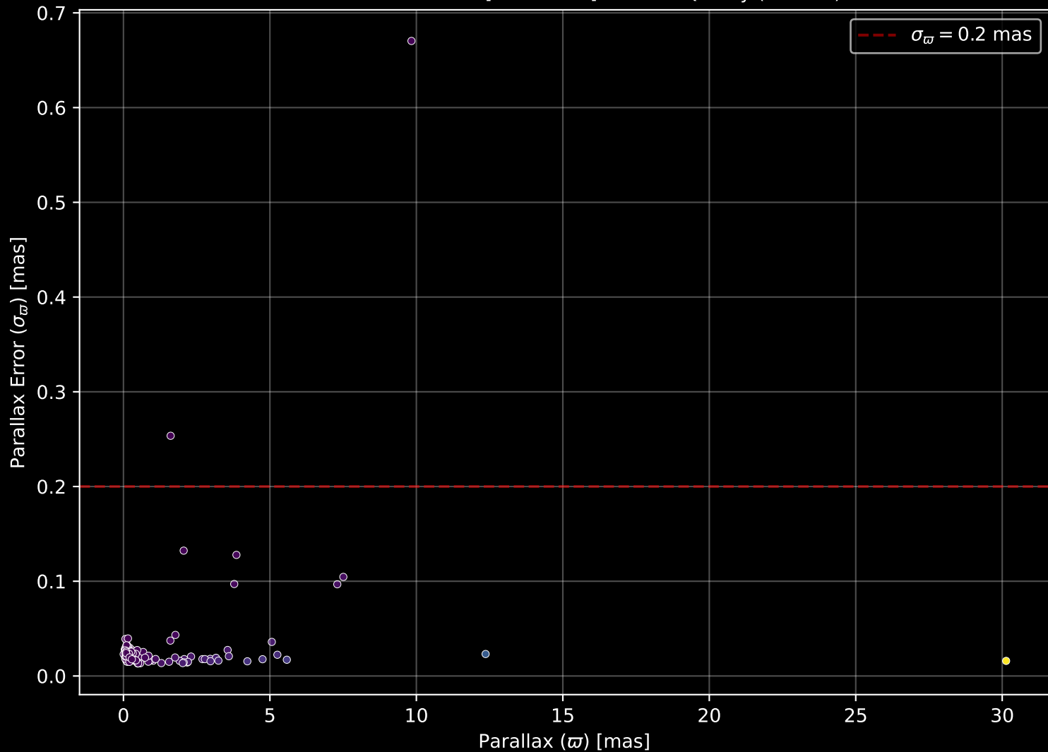
APOGEE DR17 Field: [356+12-O] Parallax Quality (n= 154)
