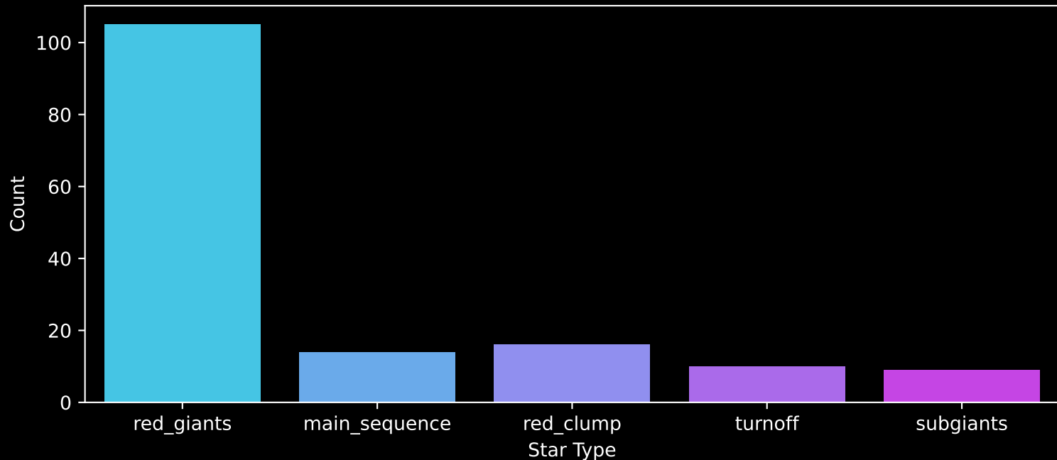
APOGEE DR17 Field: [356+12-O] Count plot of Star Type
