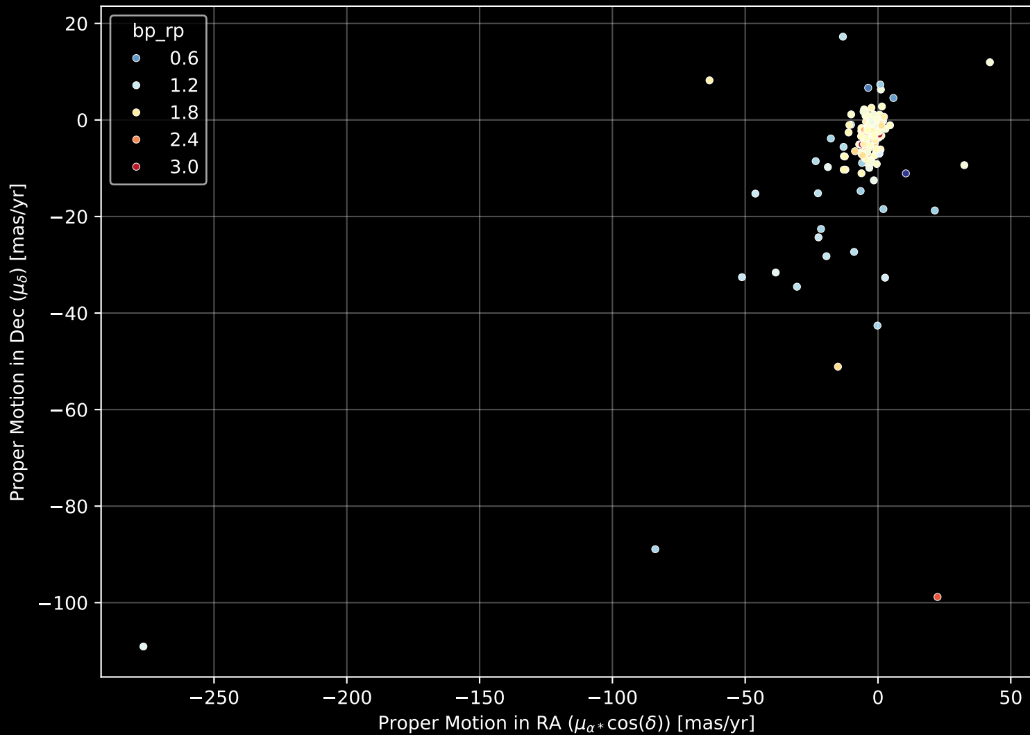
APOGEE DR17 Field: [356+12-O] Proper Motion Diagram (n= 154)
